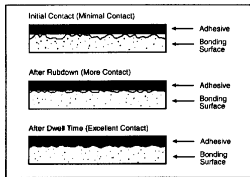
Adhesive Surface Contact
